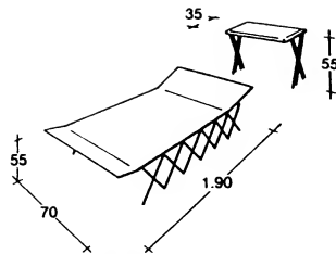
2 Canvas bed; folds to give a stool
